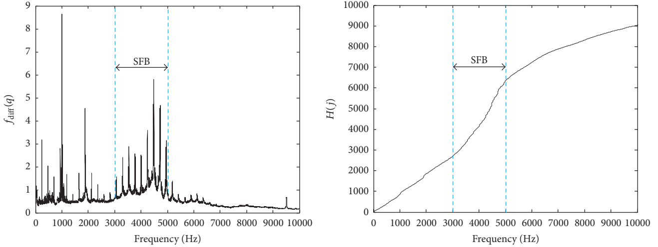
FIGURE 7: f_{\text{diff}}(q) and H(j) of Dataset 2 Bearing 1.
